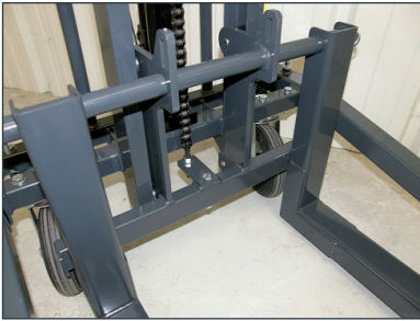
Adjustable fork sideways and easily removable, without tools.
